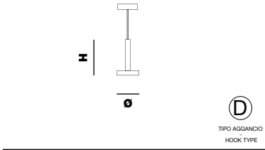
ASTRAL S1 Ø 6 cm | 2,36" H 18 cm | 7,09"
