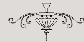
PL6 6 G9 x 40W Ø 95 cm - H 45 cm
